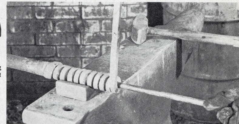
After the first section of barrel is welded, a new section of skelp is scarf-welded to the end, and another section of wrap is begun.
