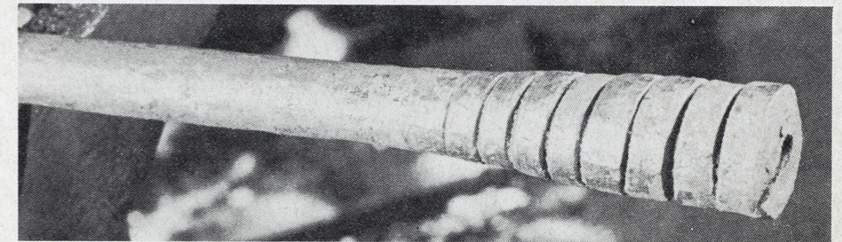
After the first section of barrel is welded, a new section of skelp is scarf-welded to the end, and another section of wrap is begun.
