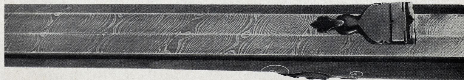
Robert Griffith forged this damascus barrel, of both twisted and untwisted piles. Twisted piles show as "watered" patterns on the etched and
