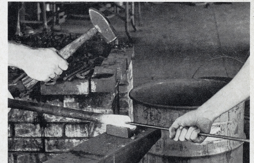
With a bottom fuller in the hardy hole, the weld is consolidated. This barrel is being formed around a mandrel; the finished barrel shown on a preceding page was forged solid, then given a hot twist full-length.
